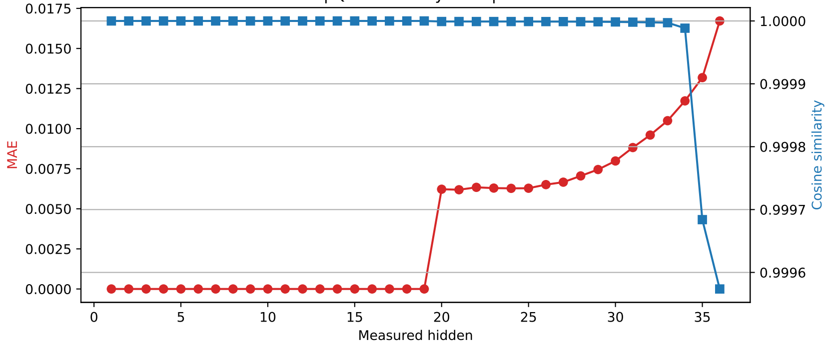
SmolLM3-3B | Quantized layer 19 | float32 → int8
