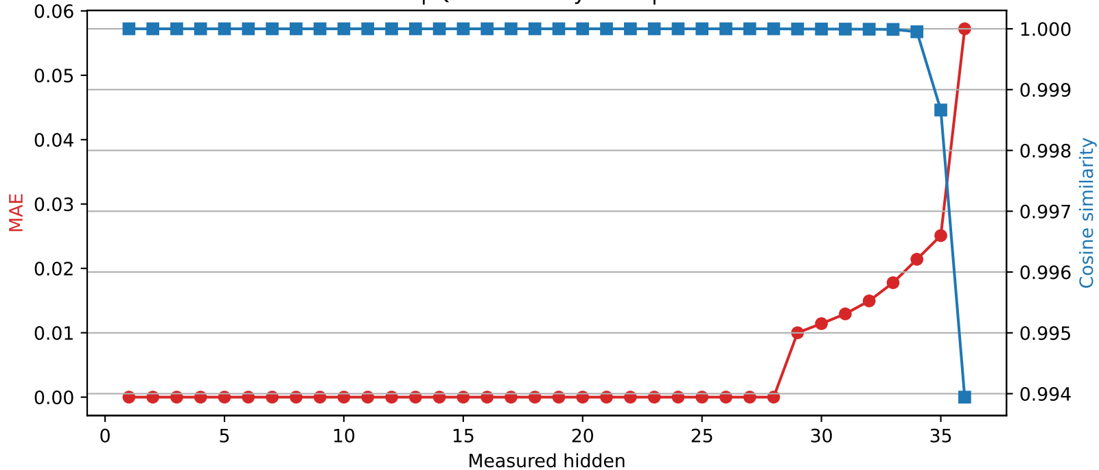
SmolLM3-3B | Quantized layer 28 | float64 → int8
