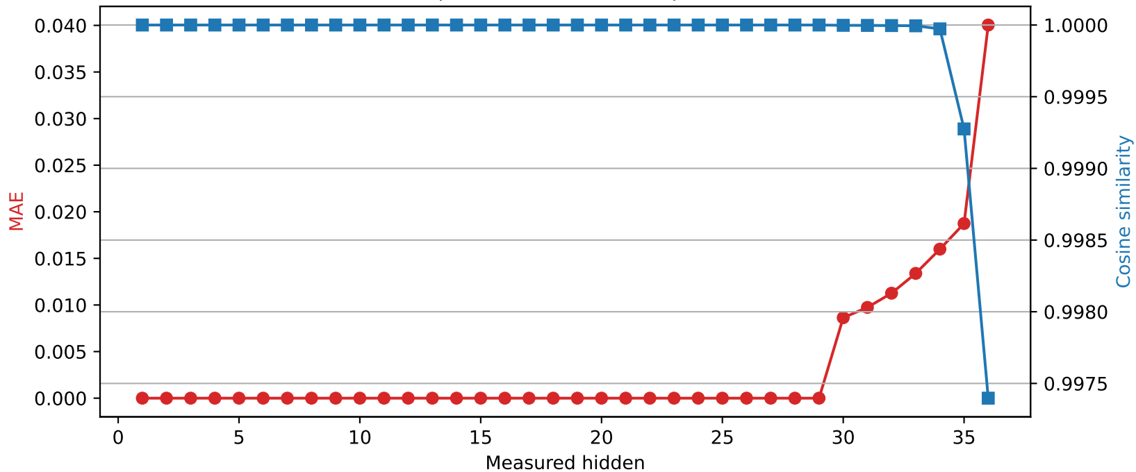
SmolLM3-3B | Quantized layer 29 | float64 → int8
