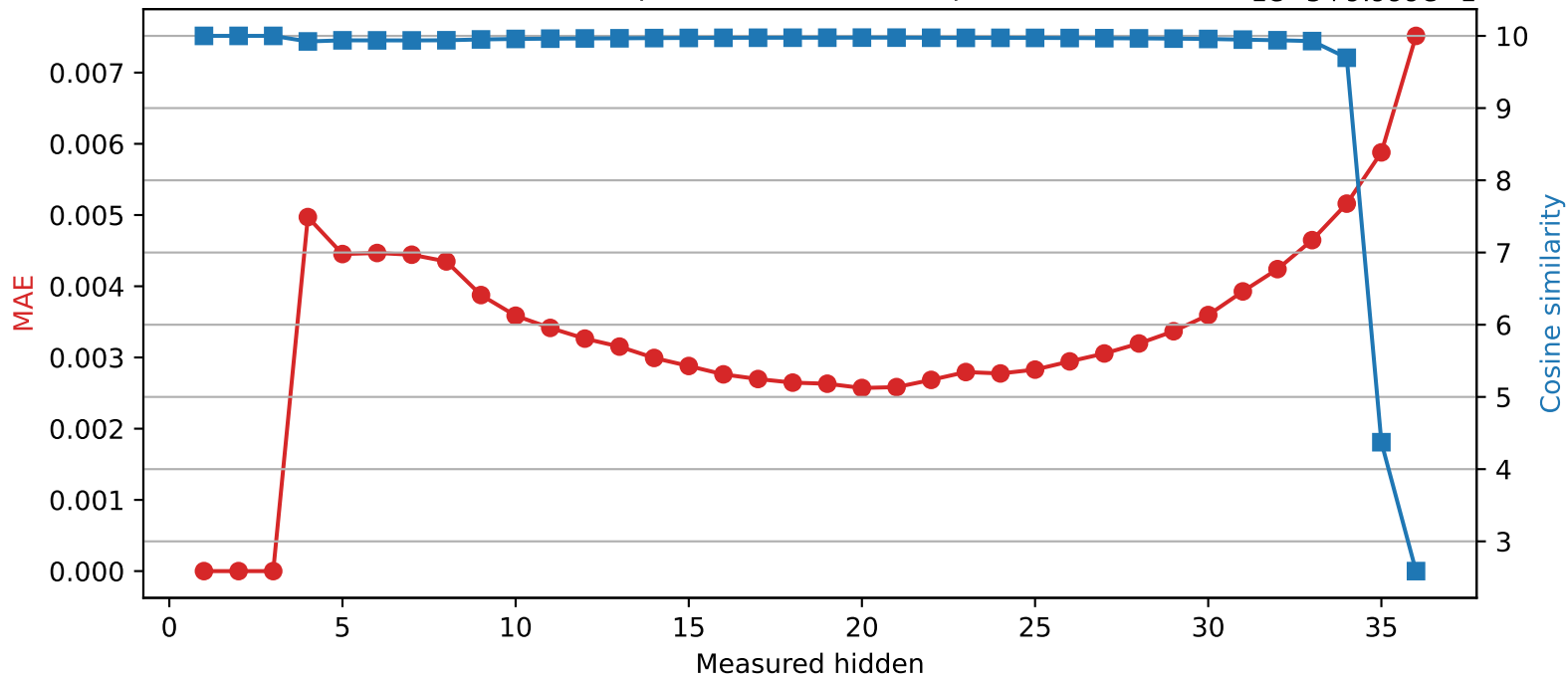
SmolLM3-3B | Quantized layer 3 | float64 → int8
