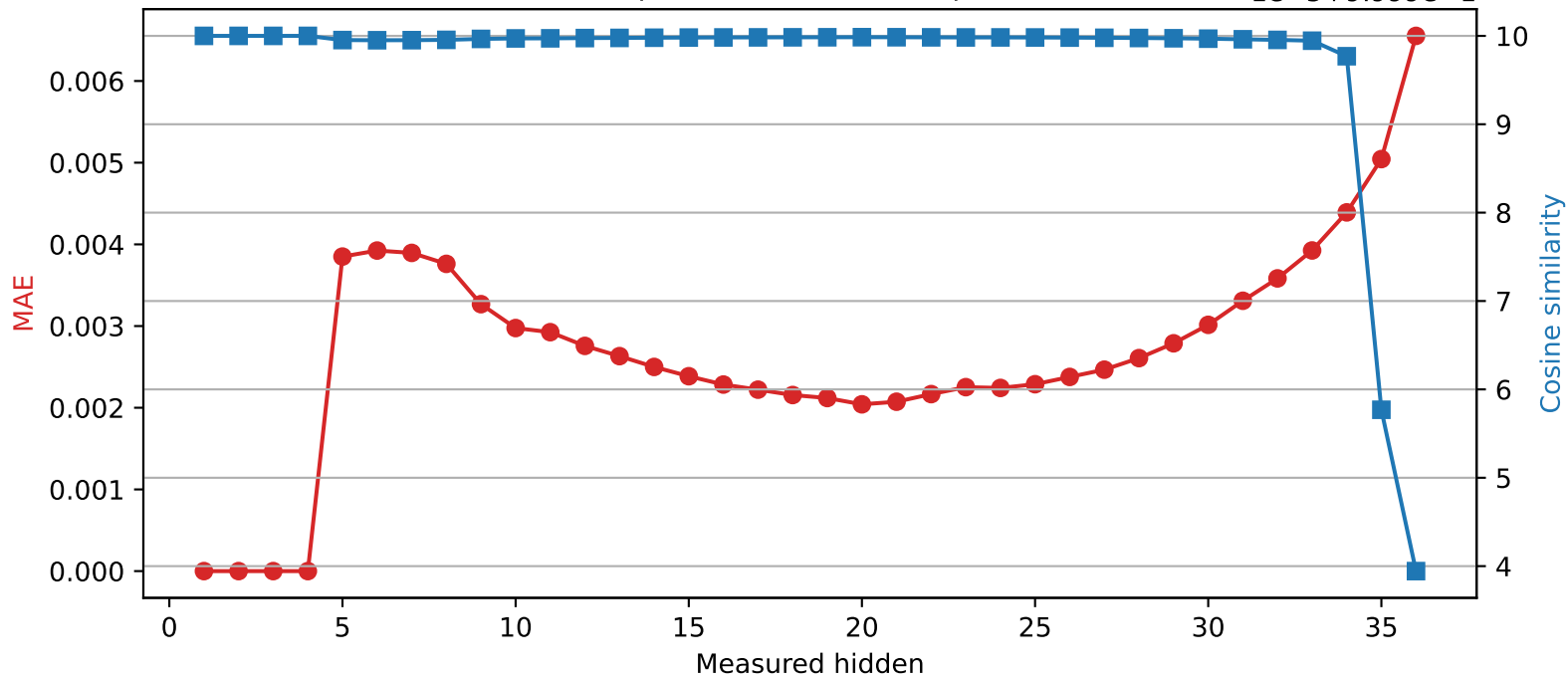
SmolLM3-3B | Quantized layer 4 | float64 → int8
