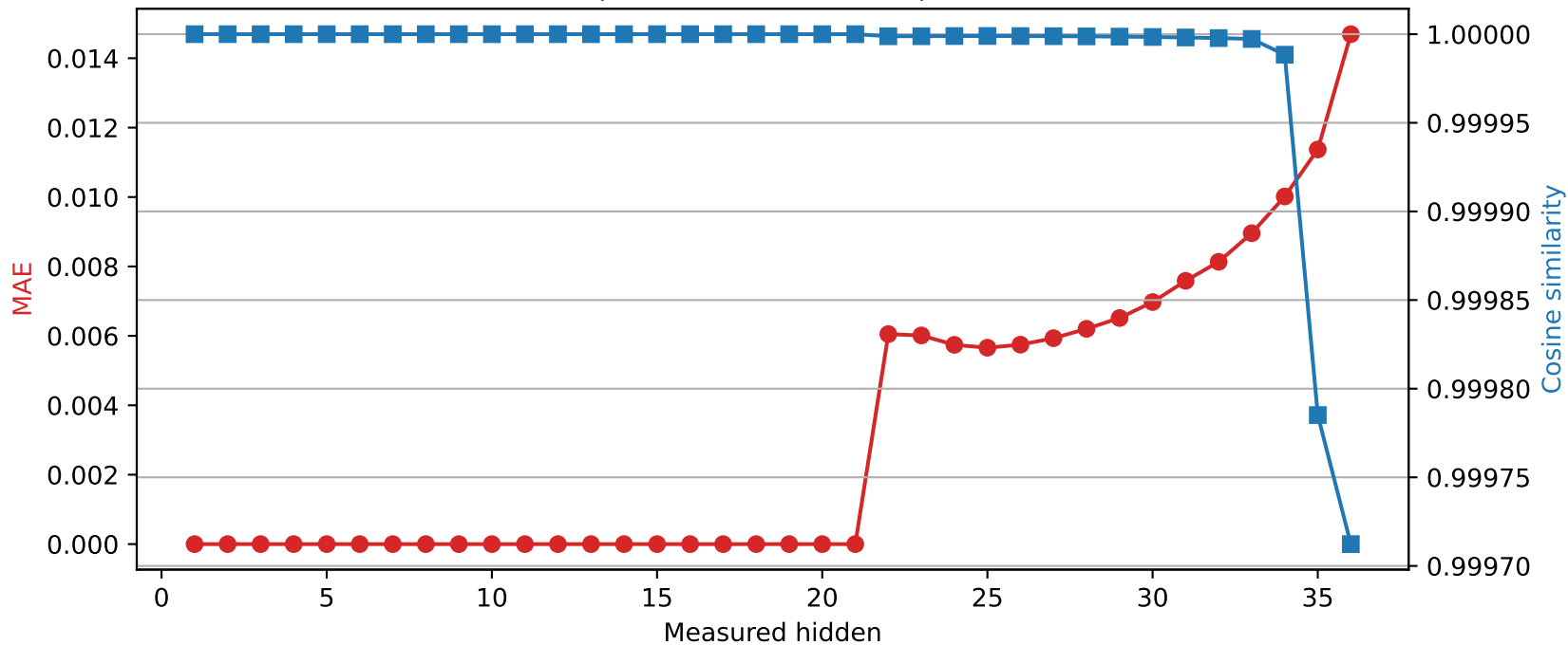
SmolLM3-3B | Quantized layer 21 | float64 → int8
