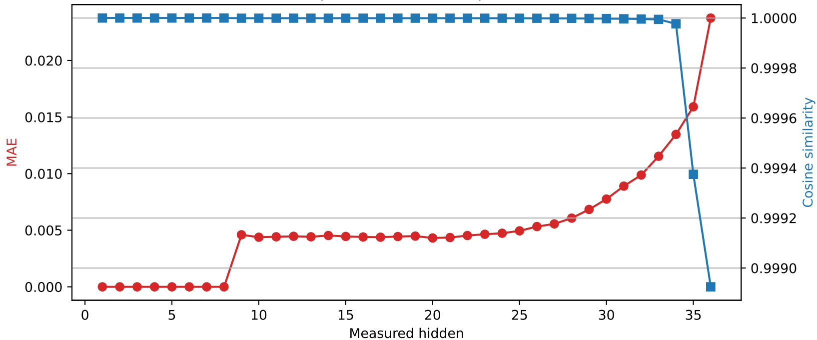
SmolLM3-3B | Quantized layer 8 | float64 → int8
