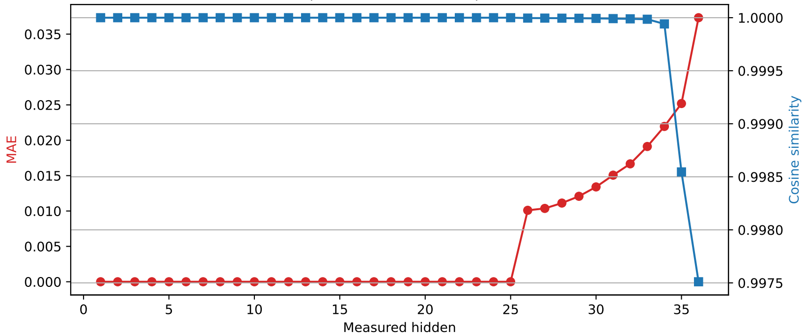
SmolLM3-3B | Quantized layer 25 | float64 → int8
