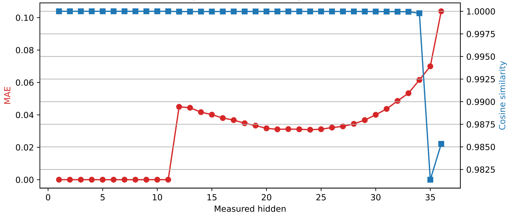
SmolLM3-3B | Quantized layer 11 | float16 → int4
