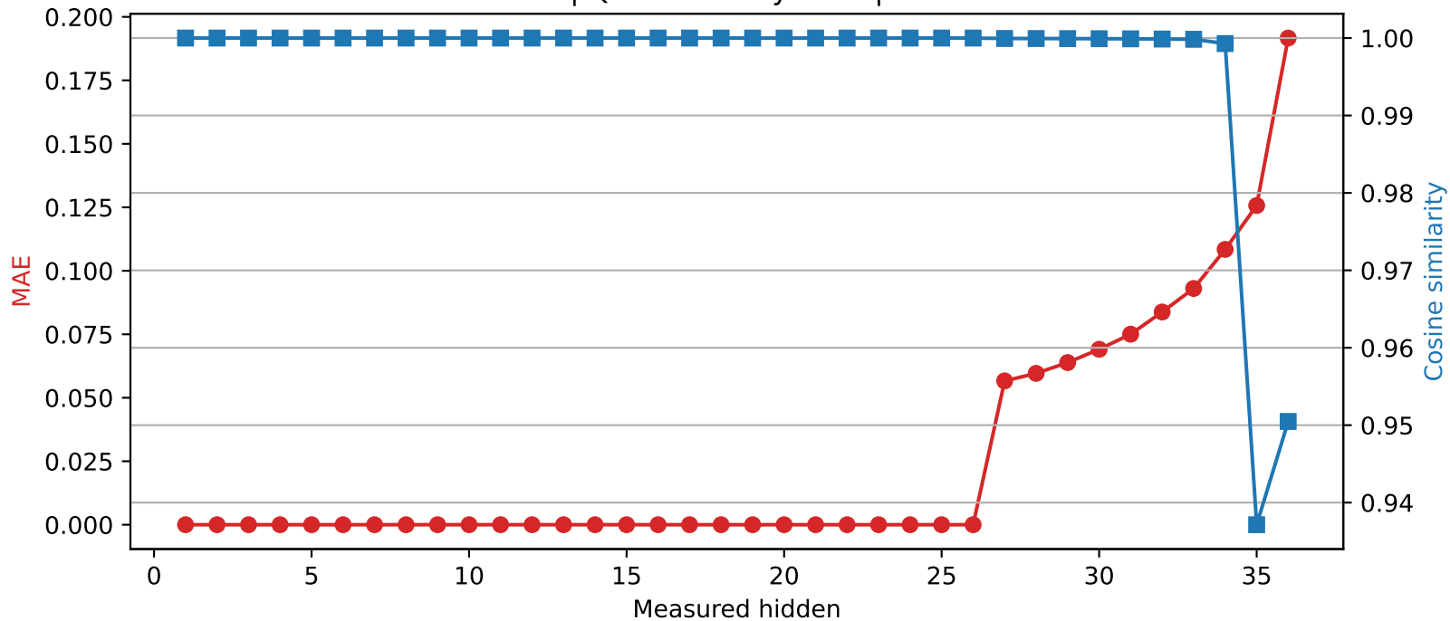
SmolLM3-3B | Quantized layer 26 | float16 → int4
