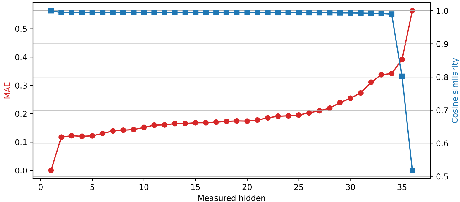
SmolLM3-3B | Quantized layer 1 | float16 \rightarrow int4
