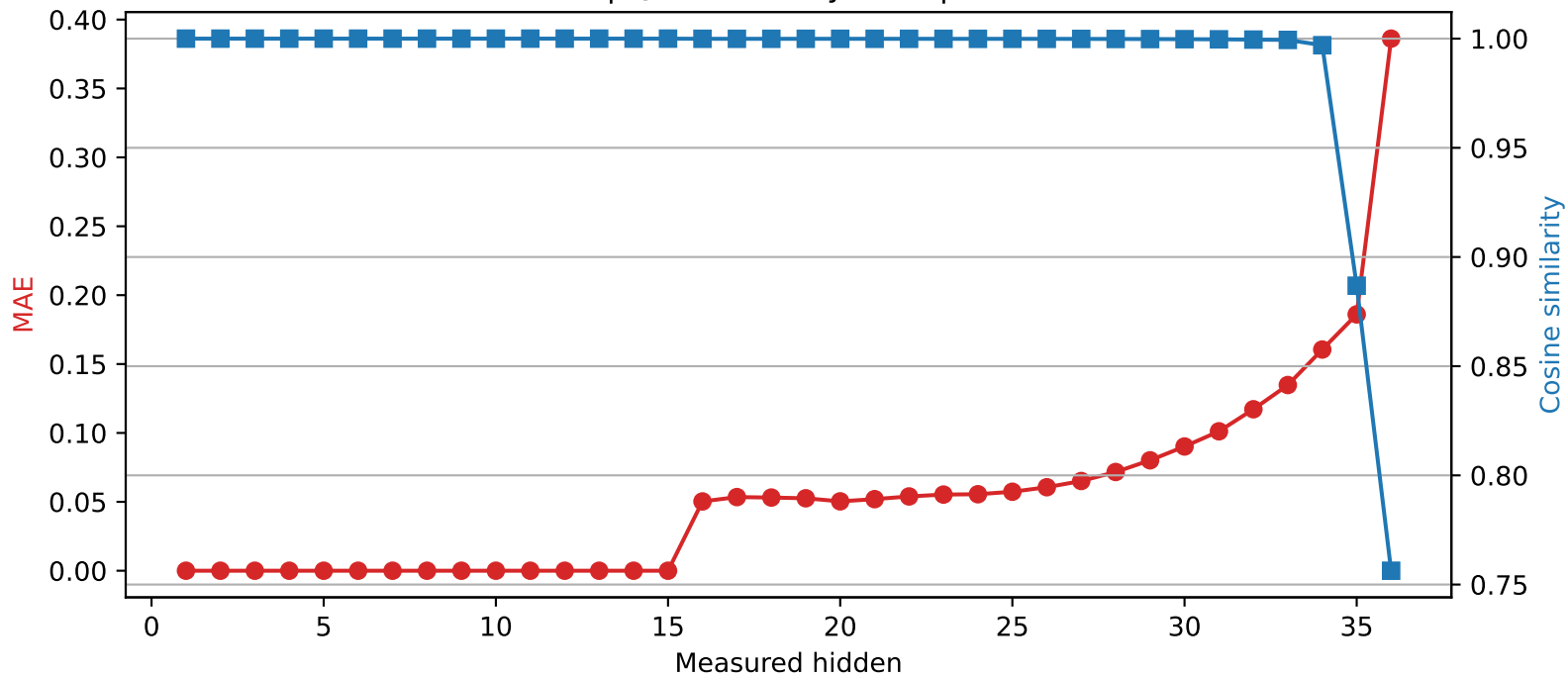
SmolLM3-3B | Quantized layer 15 | float16 → int4
