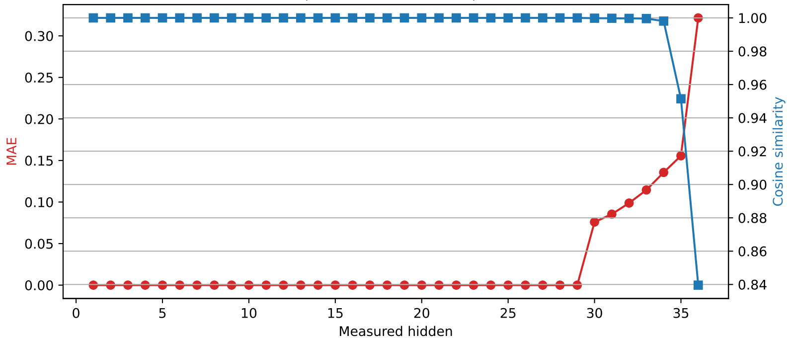
SmolLM3-3B | Quantized layer 29 | float16 → int4
