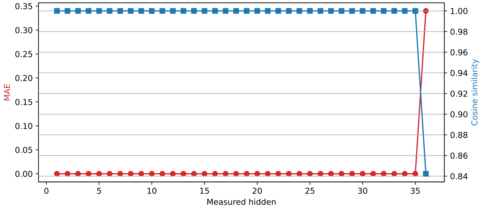
SmolLM3-3B | Quantized layer 35 | float16 \rightarrow int4
