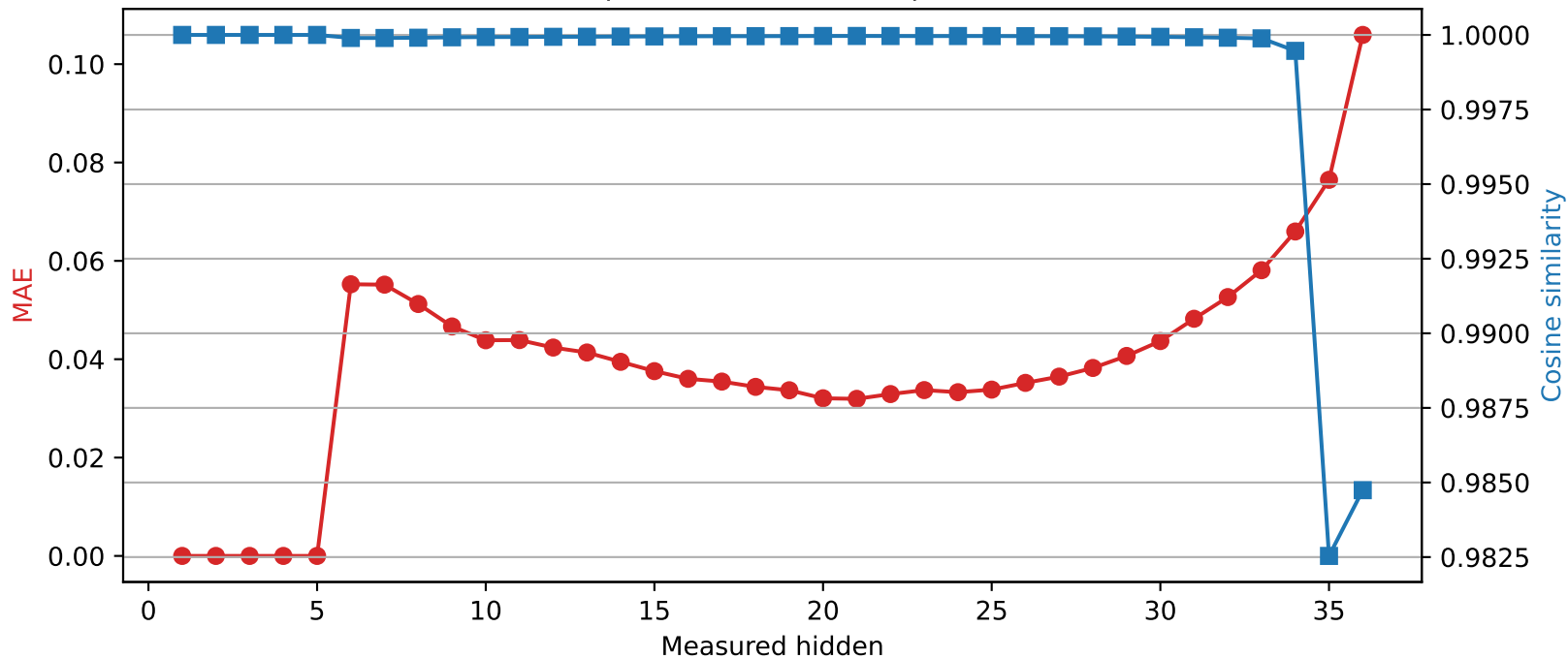
SmolLM3-3B | Quantized layer 5 | float16 → int4
