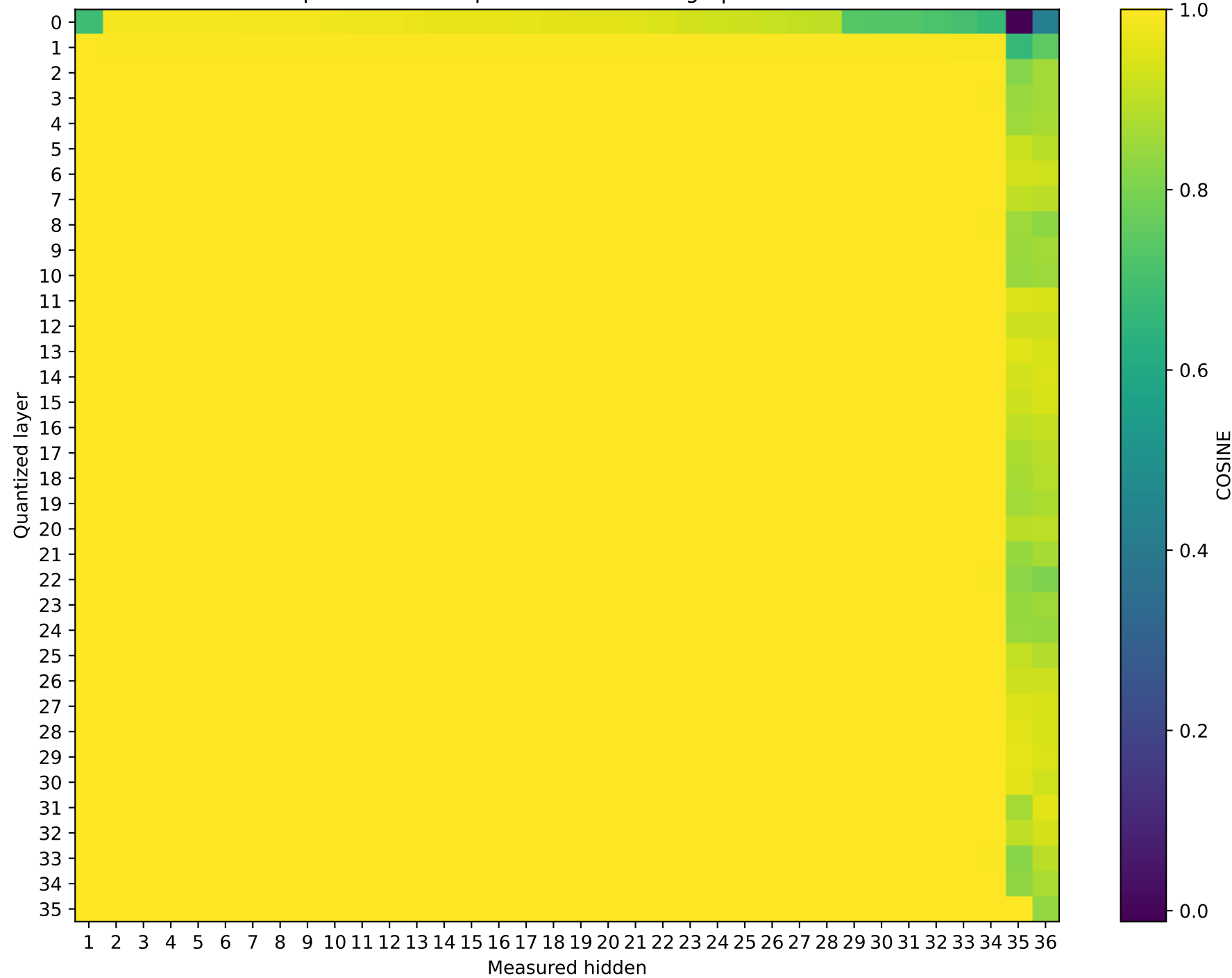
SmolLM3-3B Prompt 3: cos sim representation damage | float16 → int4
