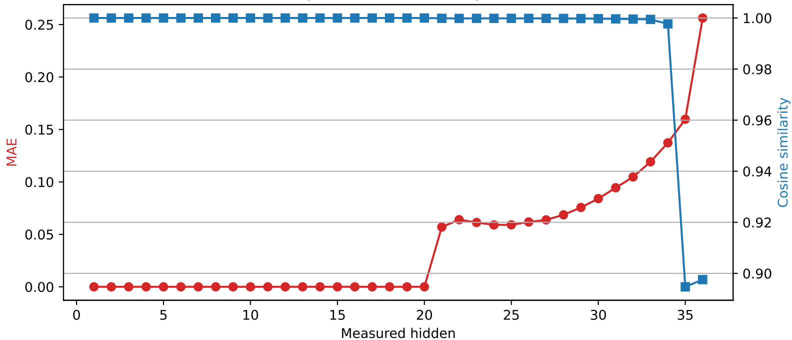
SmolLM3-3B | Quantized layer 20 | float16 → int4
