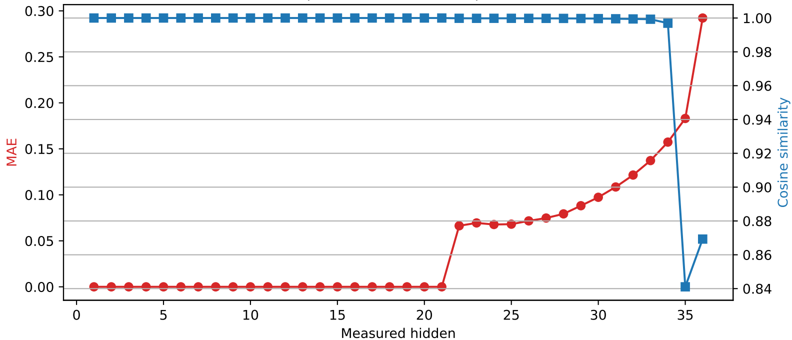
SmolLM3-3B | Quantized layer 21 | float16 \rightarrow int4
