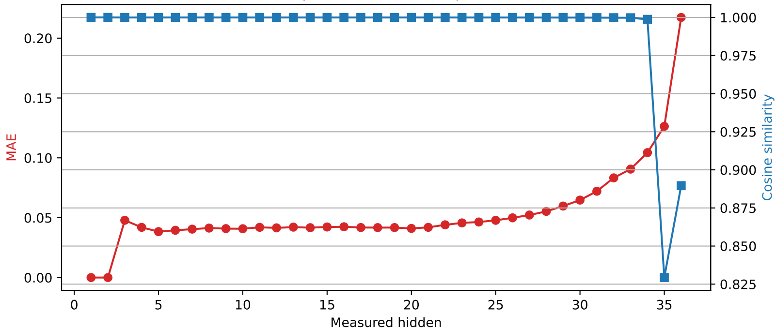
SmolLM3-3B | Quantized layer 2 | float16 \rightarrow int4
