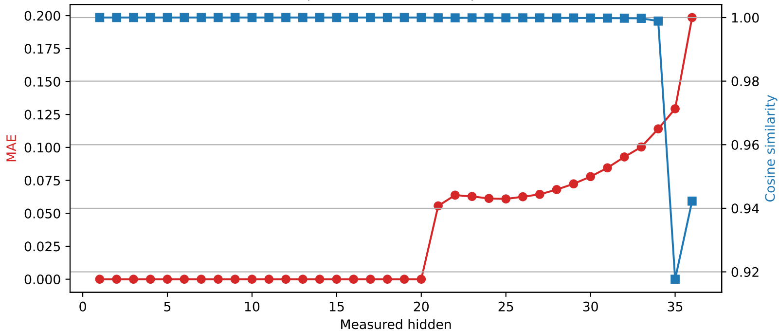
SmolLM3-3B | Quantized layer 20 | float16 \rightarrow int4
