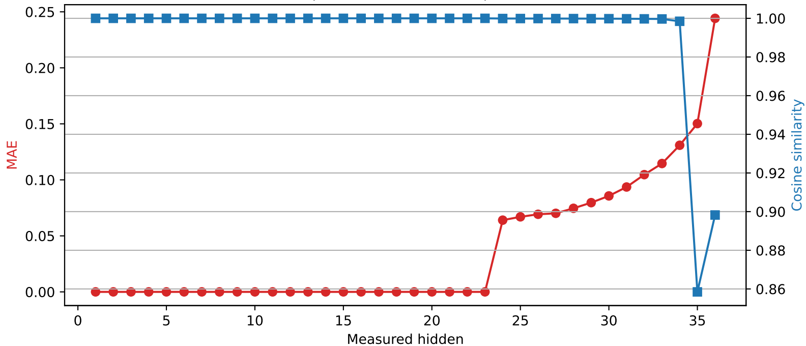
SmolLM3-3B | Quantized layer 23 | float16 \rightarrow int4
