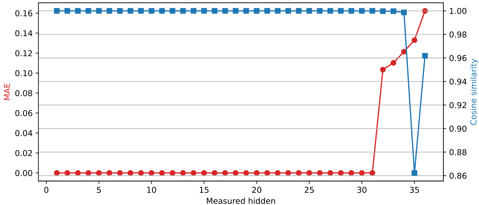
SmolLM3-3B | Quantized layer 31 | float16 \rightarrow int4
