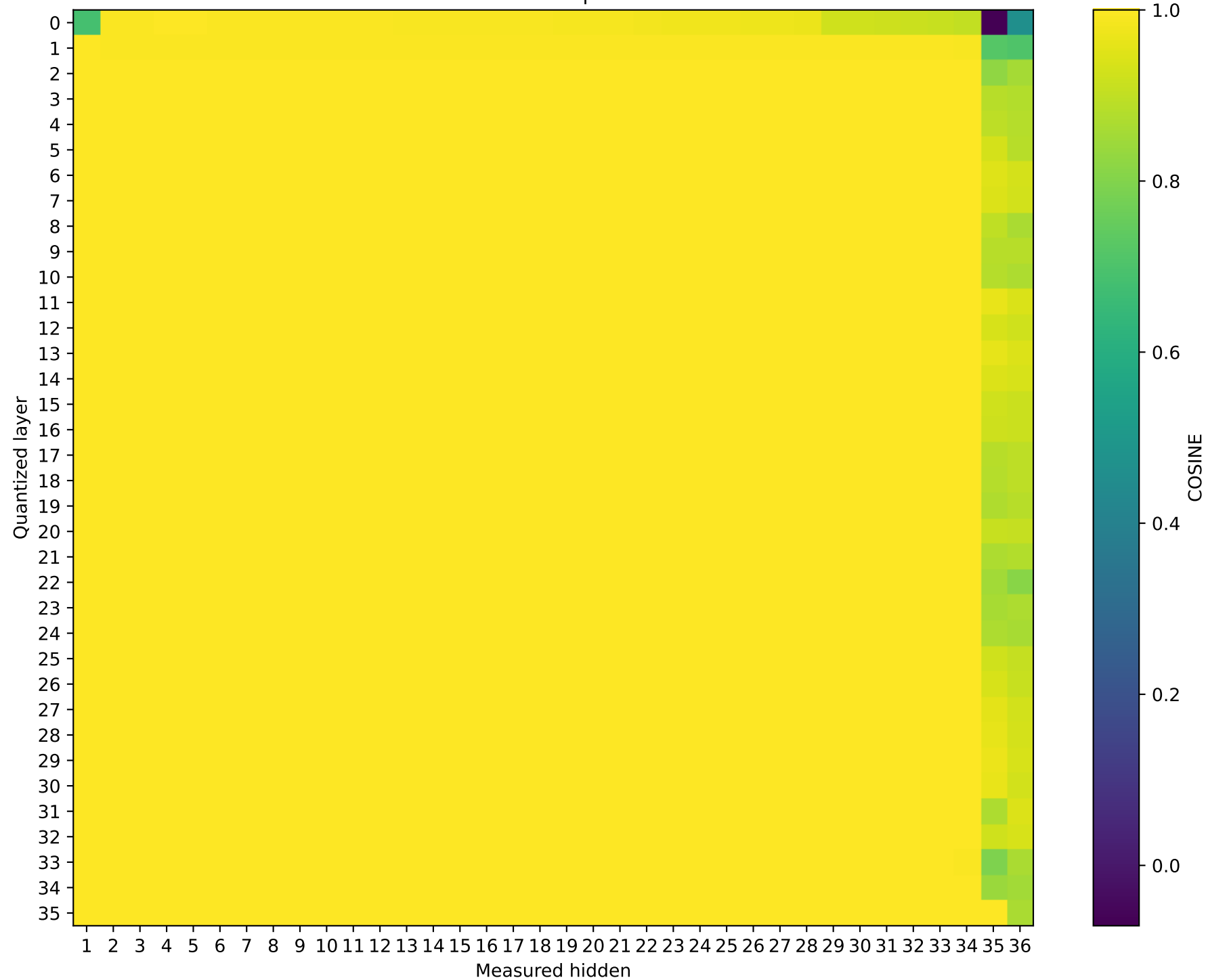
Model: SmolLM3-3B | float32 → int4
