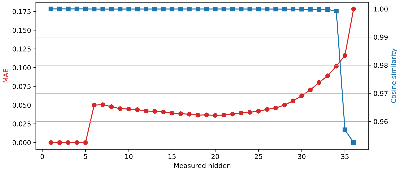
SmolLM3-3B | Quantized layer 5 | float32 → int4
