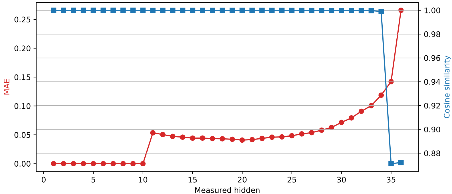
SmolLM3-3B | Quantized layer 10 | float32 \rightarrow int4
