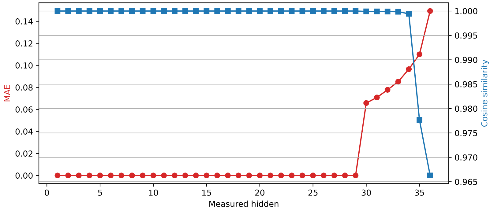
SmolLM3-3B | Quantized layer 29 | float32 → int4
