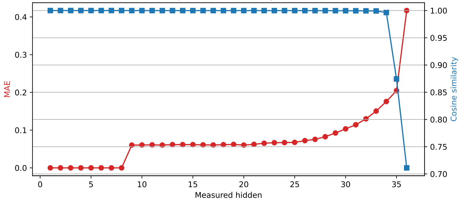
SmolLM3-3B | Quantized layer 8 | float32 → int4
