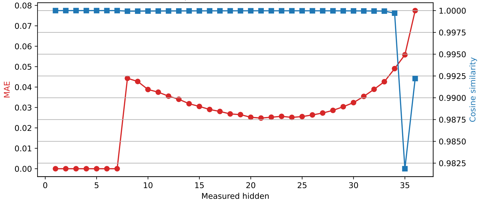
SmolLM3-3B | Quantized layer 7 | float32 → int4
