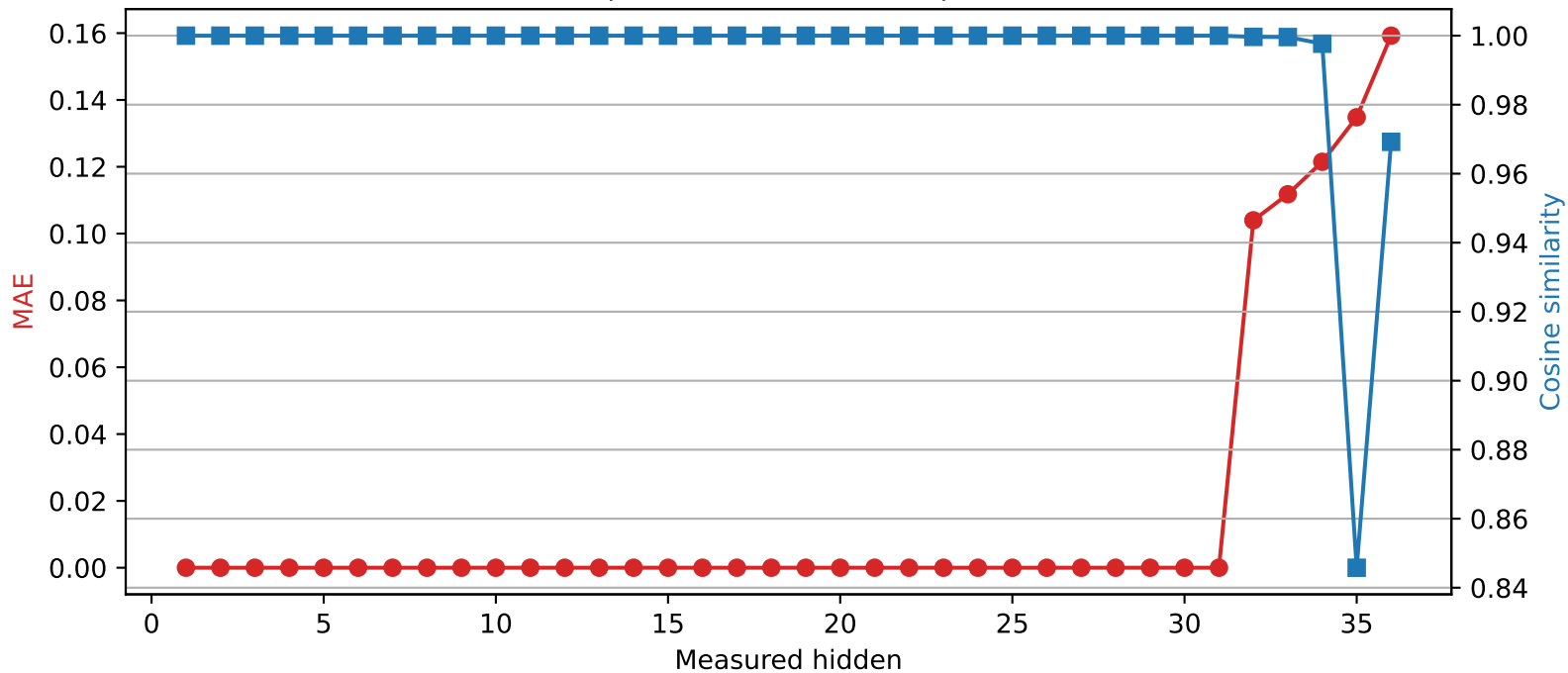
SmolLM3-3B | Quantized layer 31 | float32 → int4
