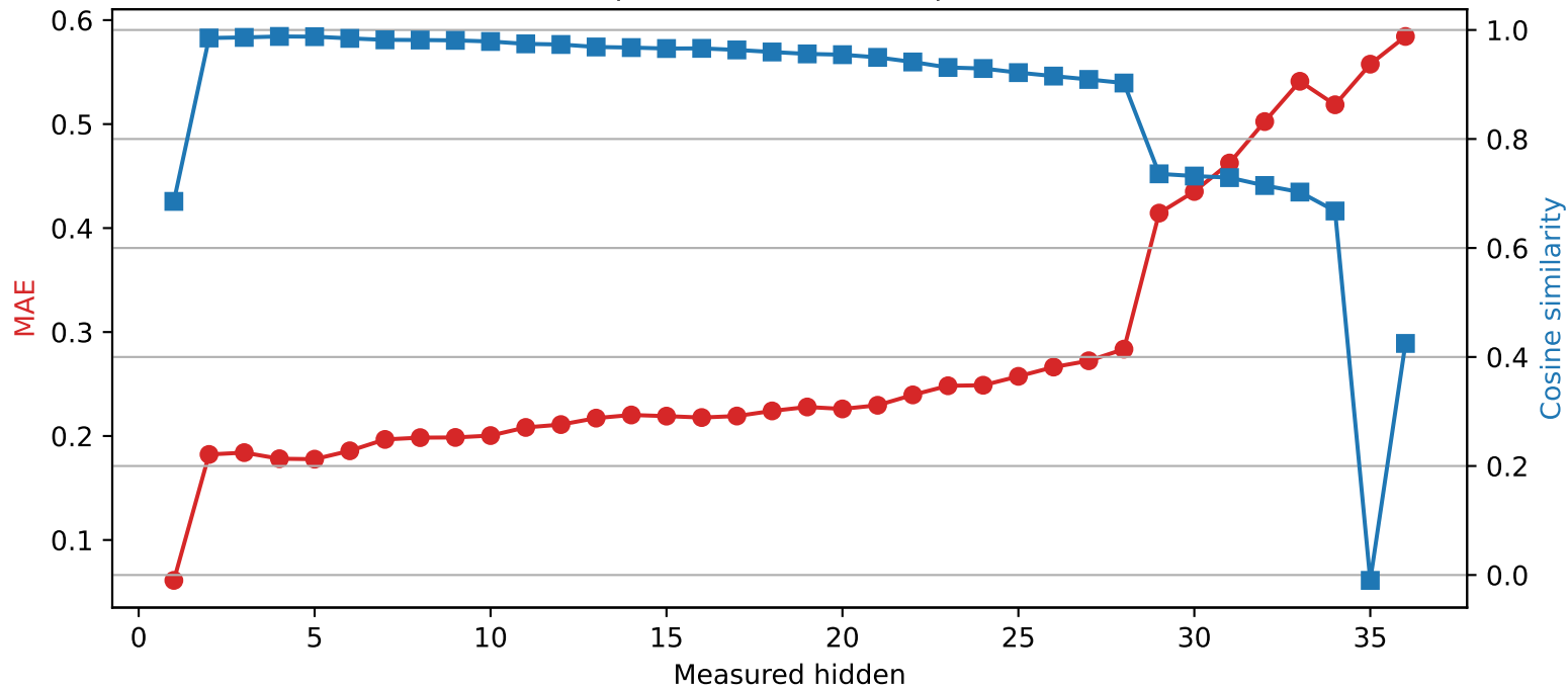
SmolLM3-3B | Quantized layer 0 | float32 \rightarrow int4
