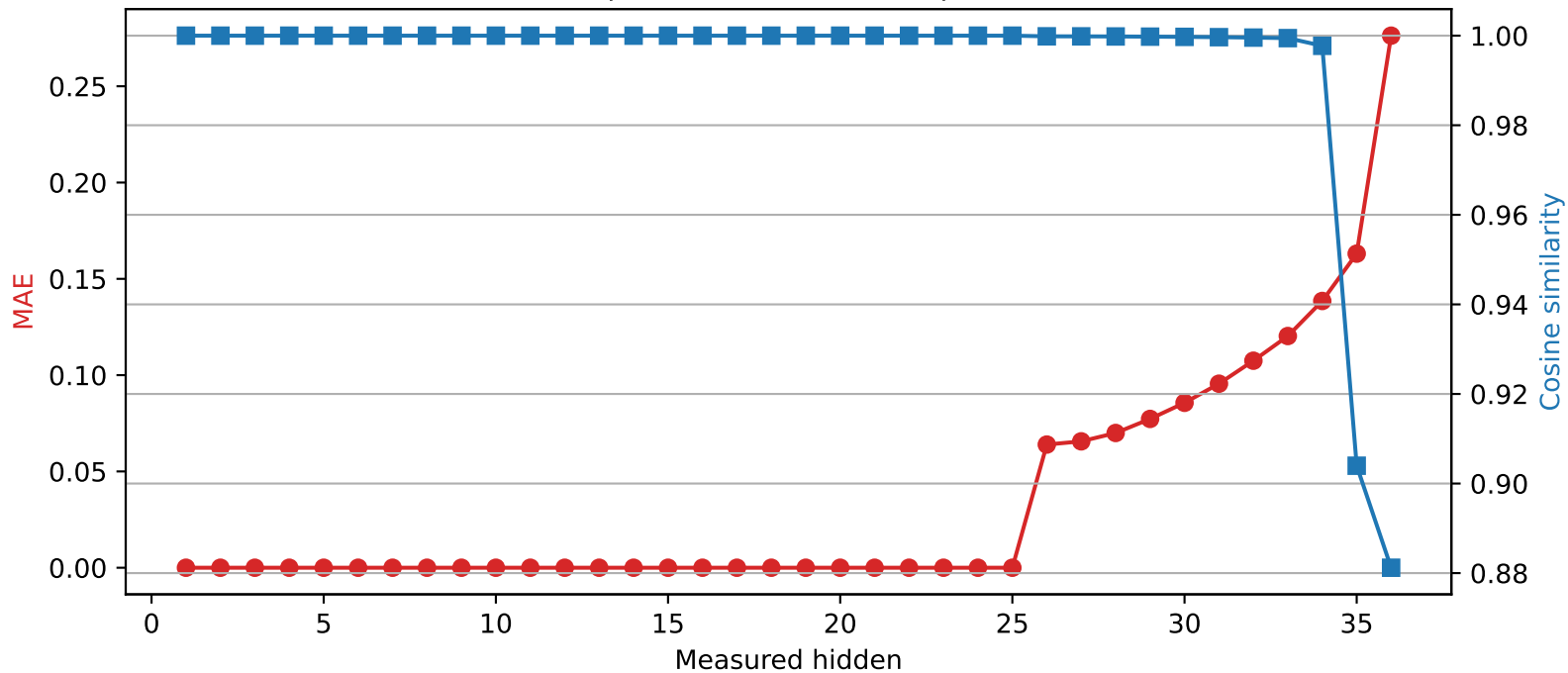
SmolLM3-3B | Quantized layer 25 | float32 → int4
