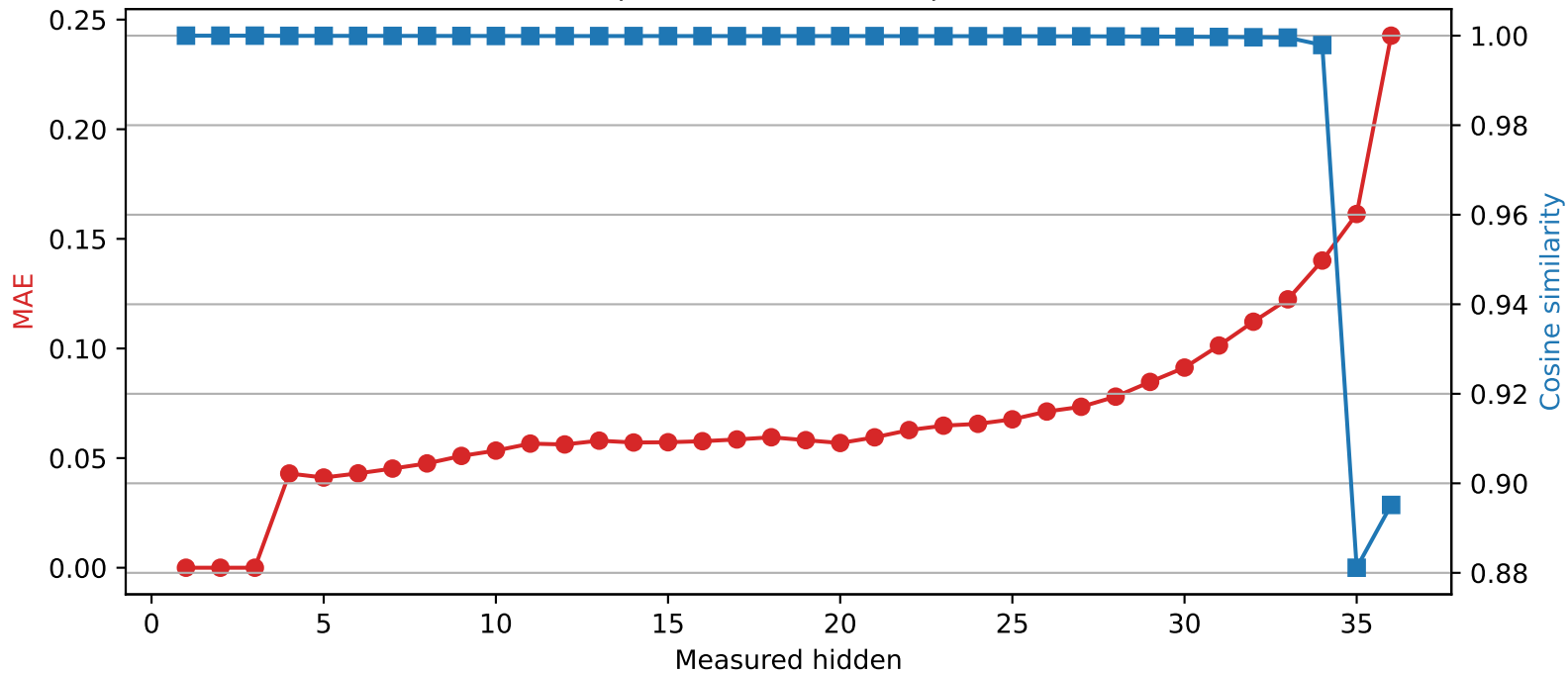
SmolLM3-3B | Quantized layer 3 | float32 → int4
