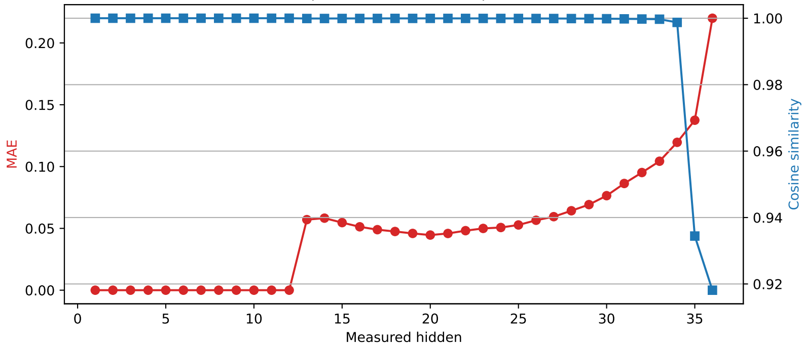
SmolLM3-3B | Quantized layer 12 | float32 \rightarrow int4
