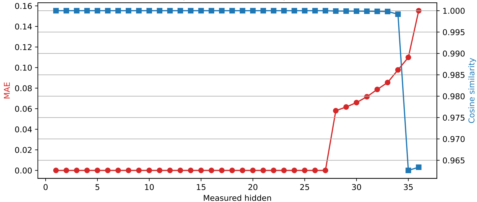
SmolLM3-3B | Quantized layer 27 | float32 → int4
