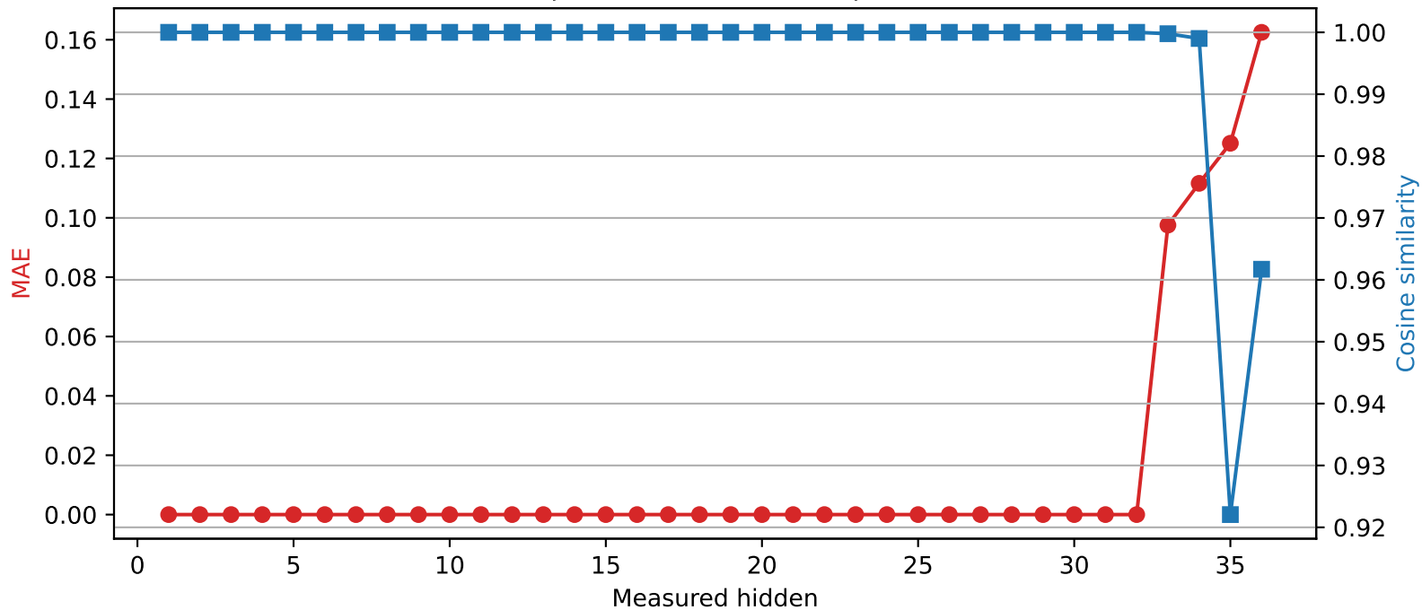
SmolLM3-3B | Quantized layer 32 | float32 → int4
