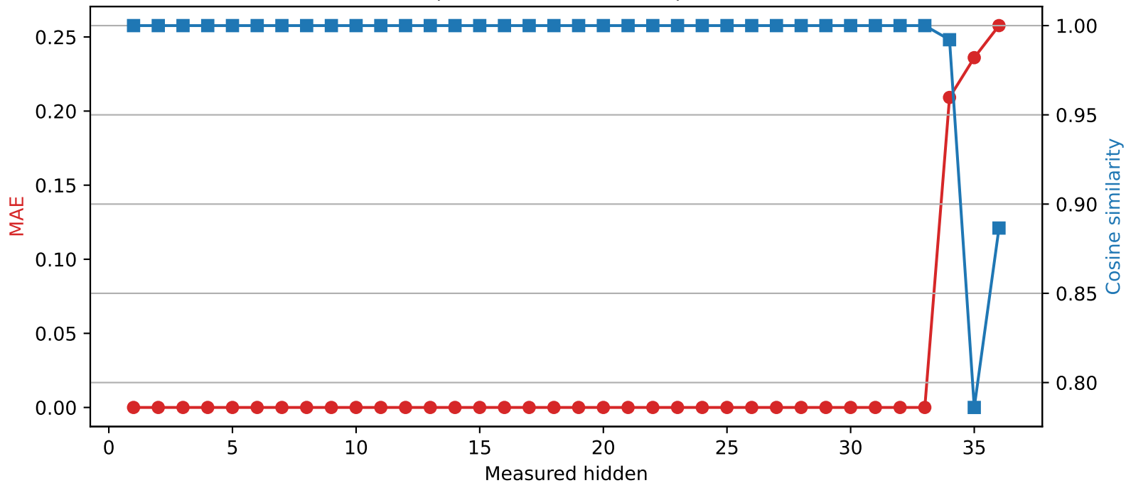
SmolLM3-3B | Quantized layer 33 | float32 \rightarrow int4
