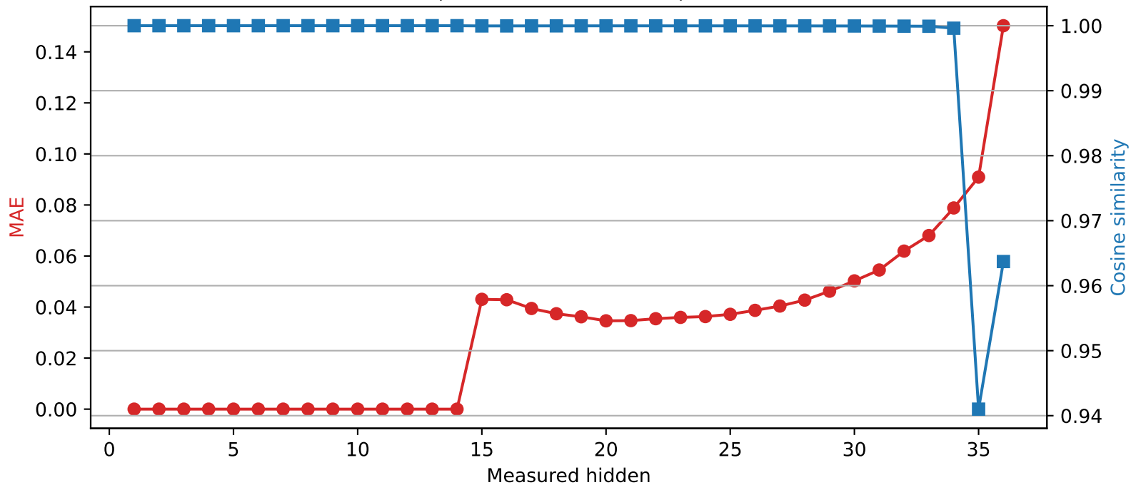
SmolLM3-3B | Quantized layer 14 | float64 → int4
