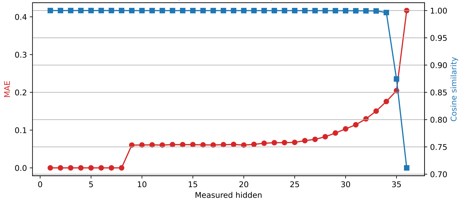
SmolLM3-3B | Quantized layer 8 | float64 → int4
