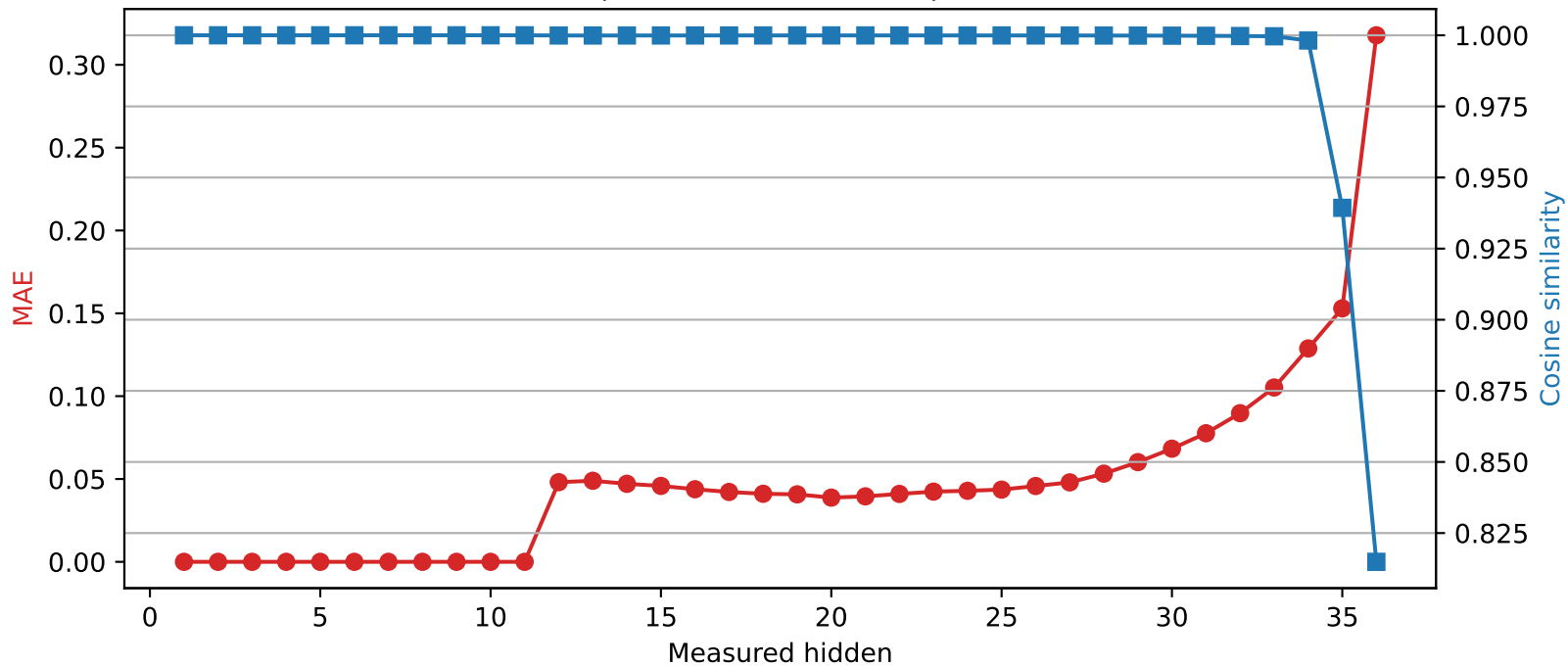
SmolLM3-3B | Quantized layer 11 | float64 → int4
