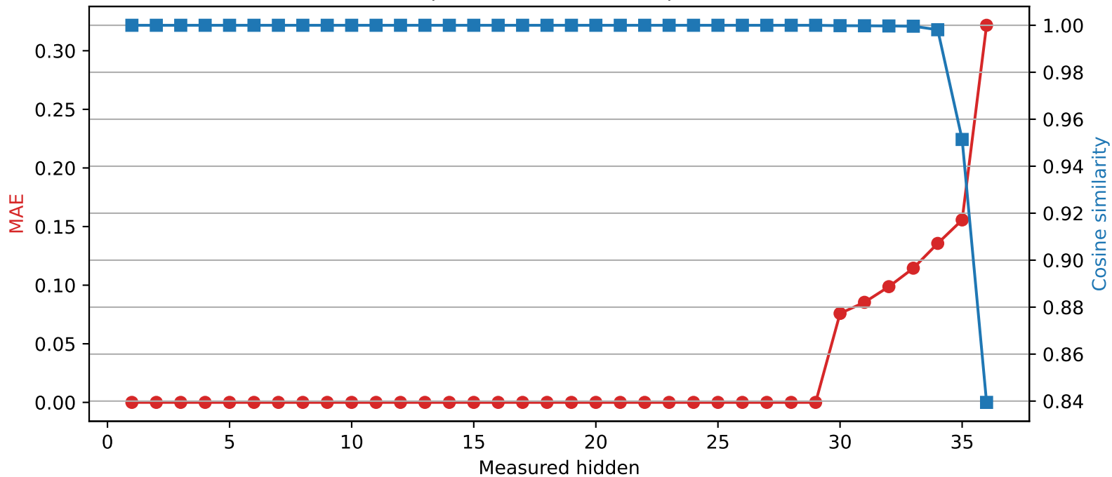
SmolLM3-3B | Quantized layer 29 | float64 → int4
