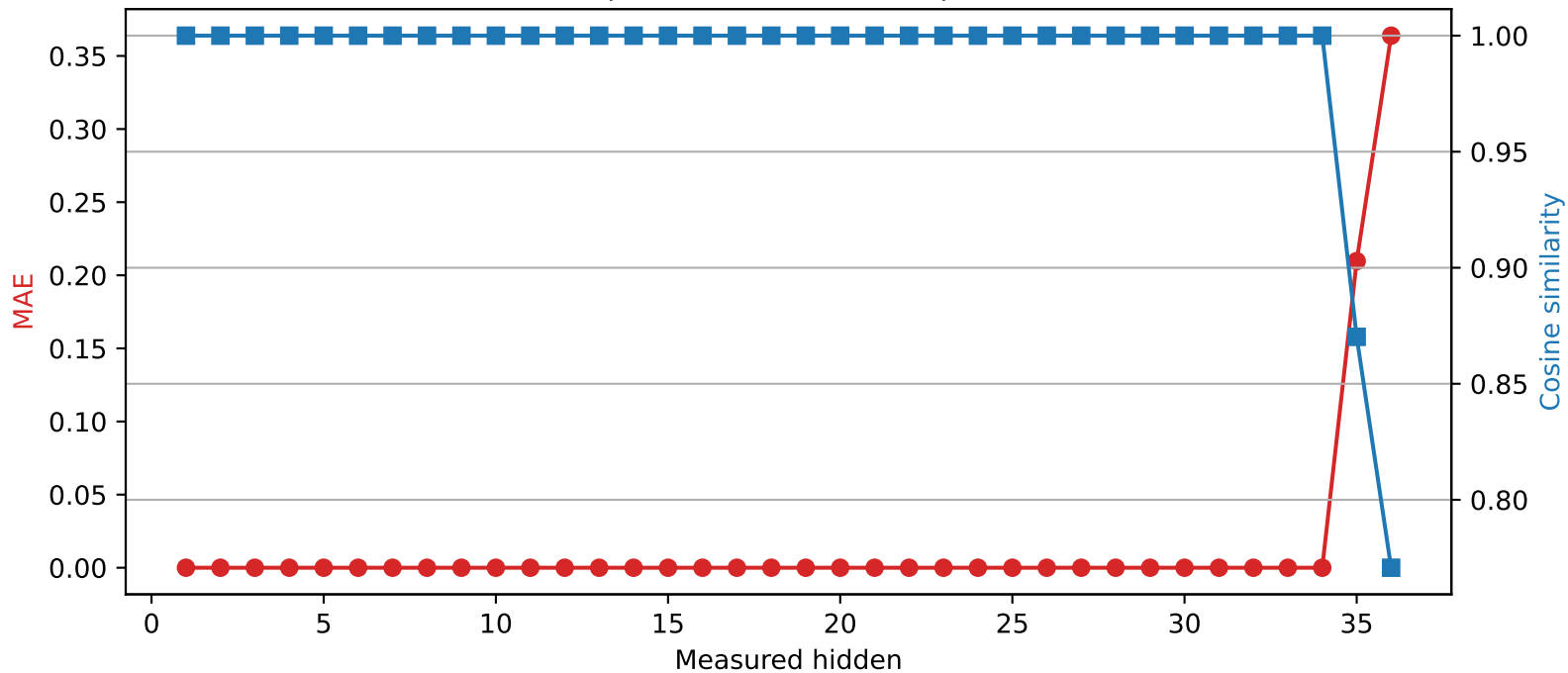
SmolLM3-3B | Quantized layer 34 | float64 → int4
