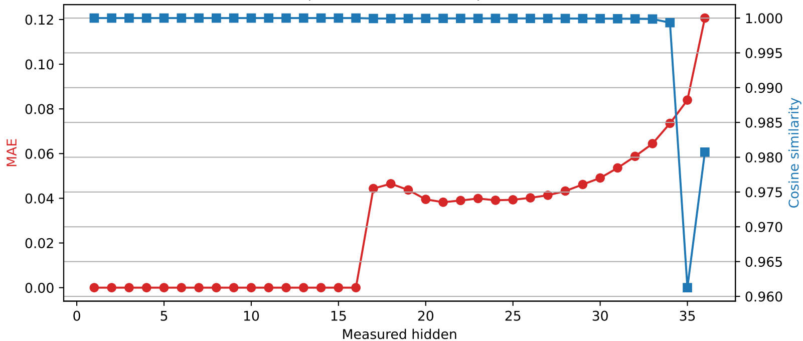
SmolLM3-3B | Quantized layer 16 | float64 → int4
