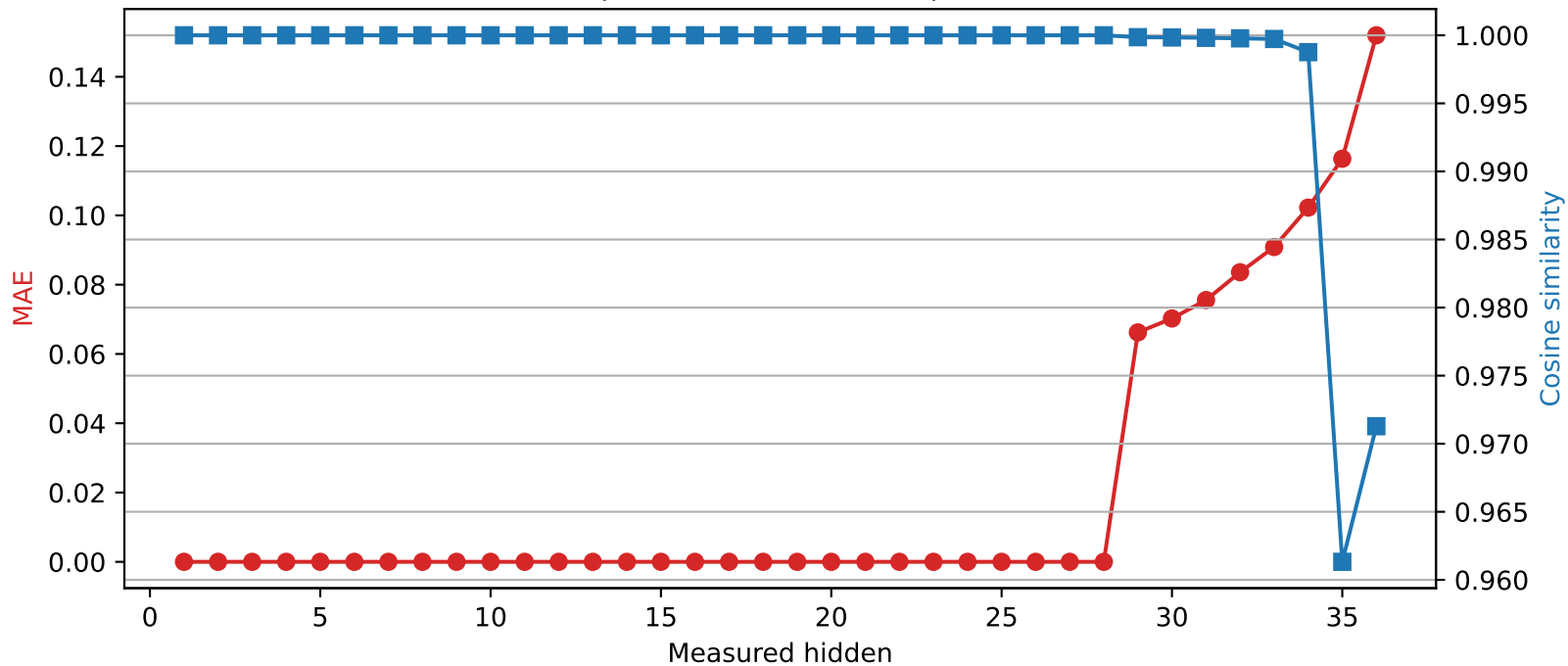
SmolLM3-3B | Quantized layer 28 | float64 → int4
