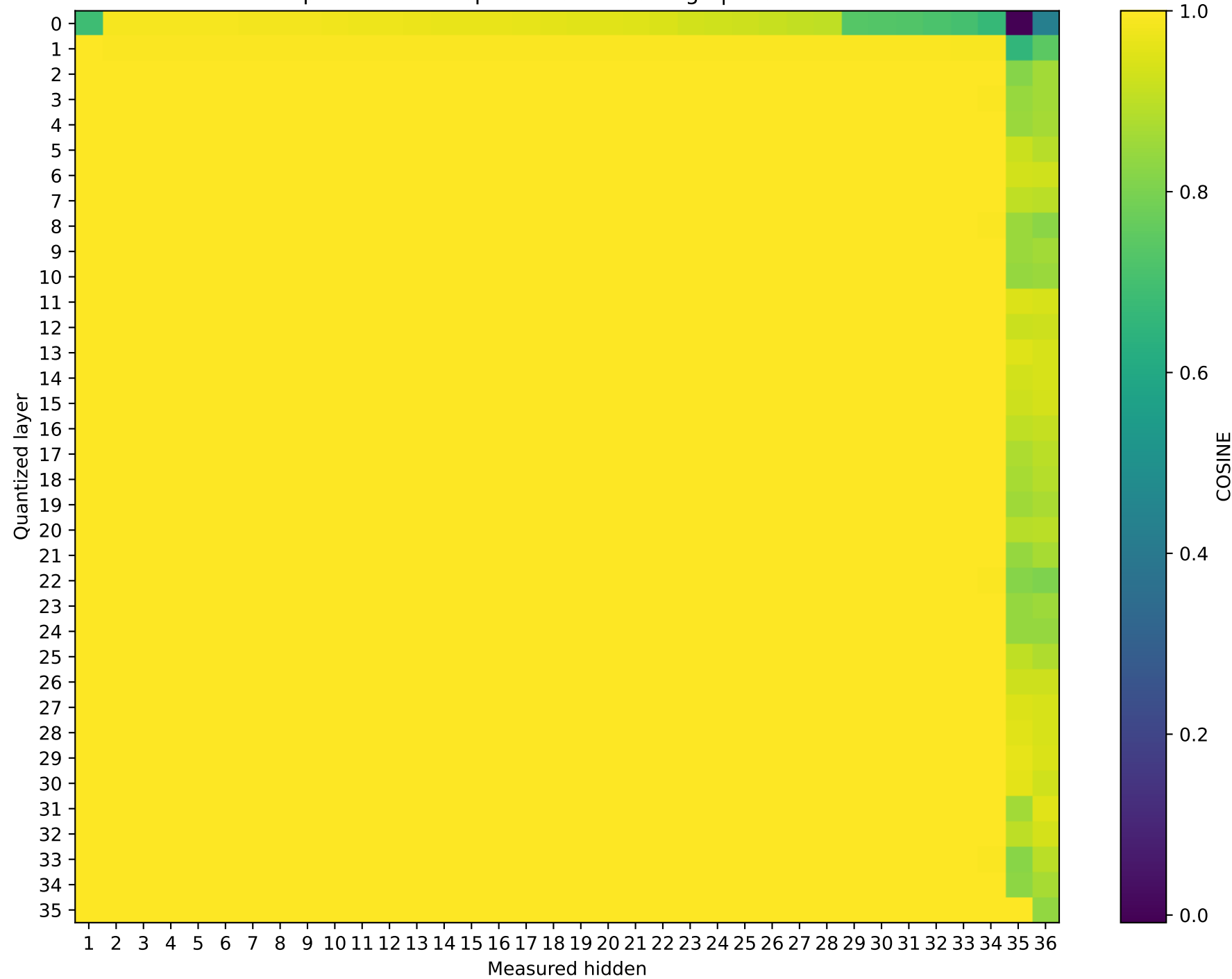
SmolLM3-3B Prompt 3: cos sim representation damage | float64 → int4
