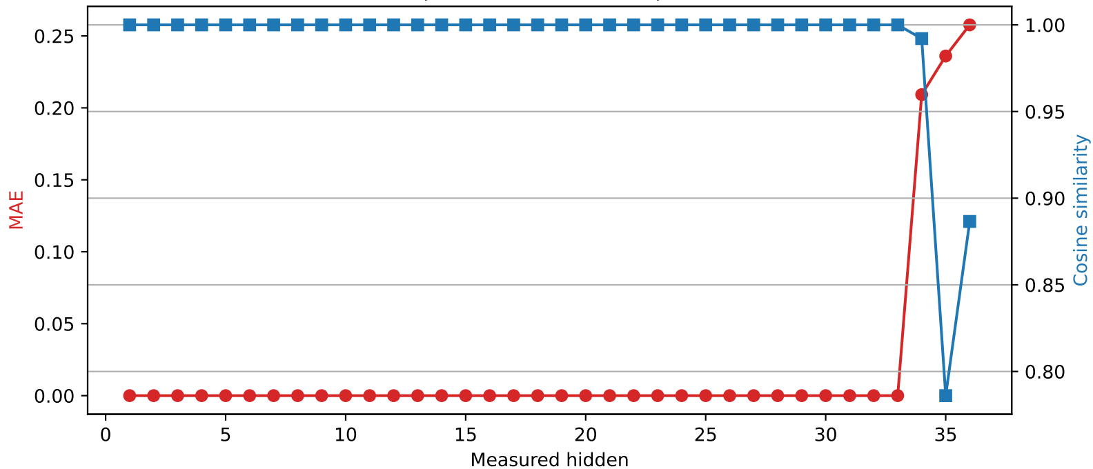
SmolLM3-3B | Quantized layer 33 | float64 → int4
