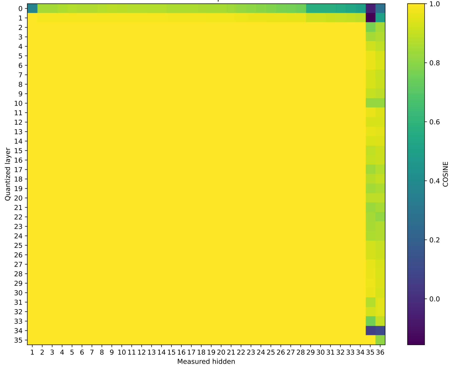
Model: SmolLM3-3B | float16 → int2
