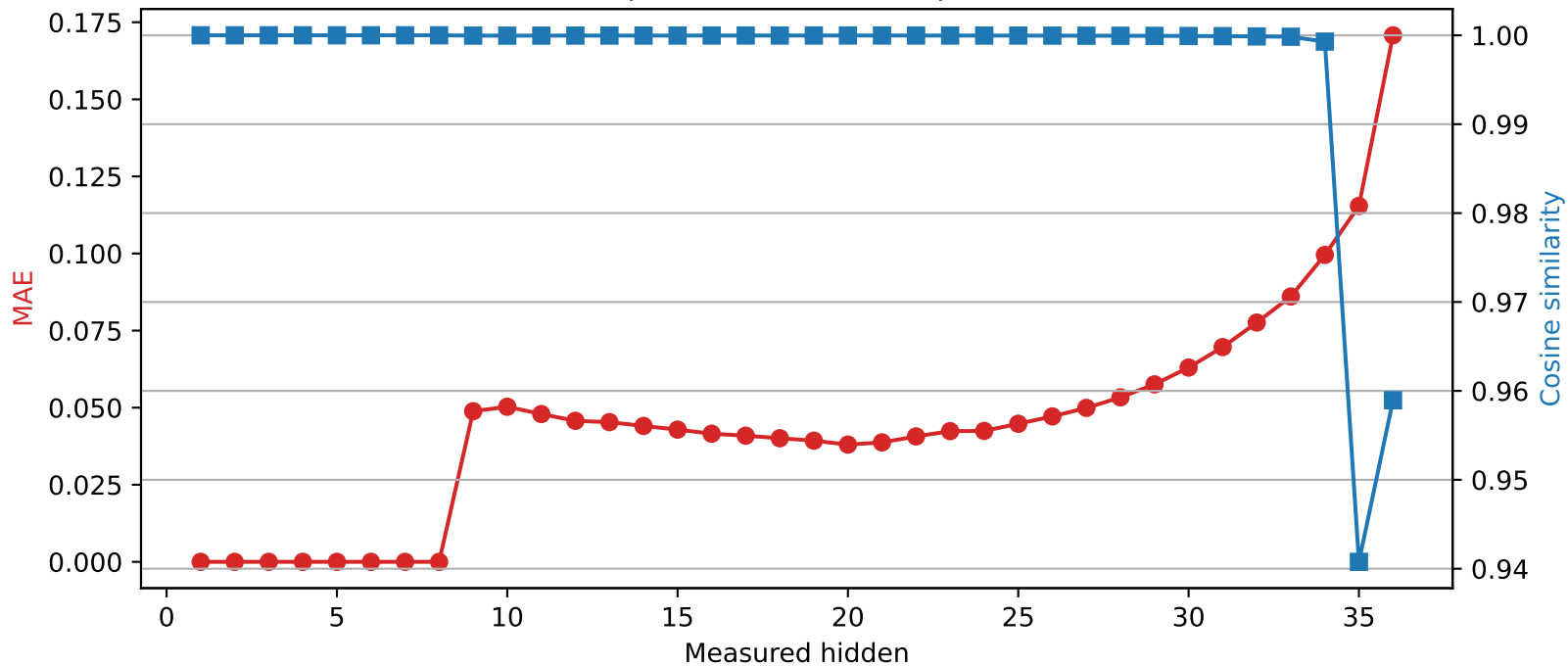
SmolLM3-3B | Quantized layer 8 | float16 \rightarrow int2
