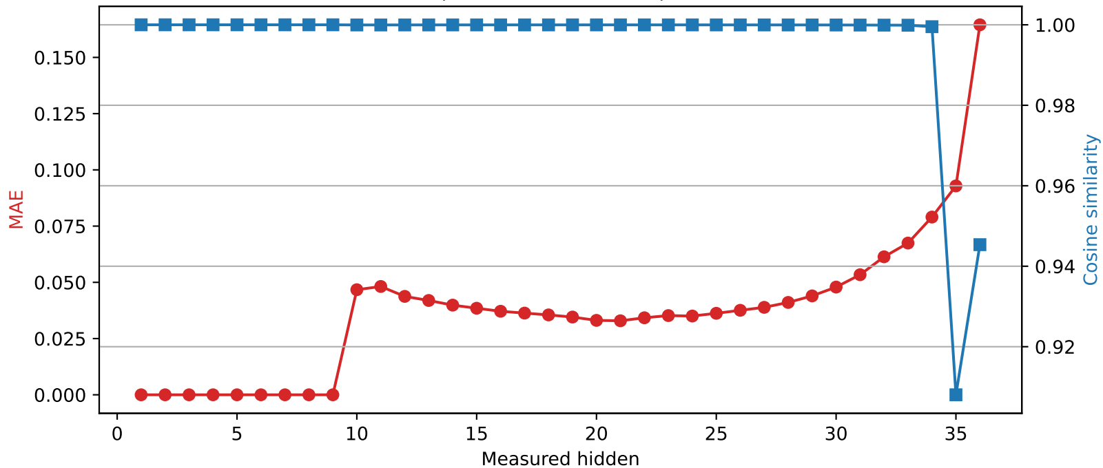
SmolLM3-3B | Quantized layer 9 | float16 → int2
