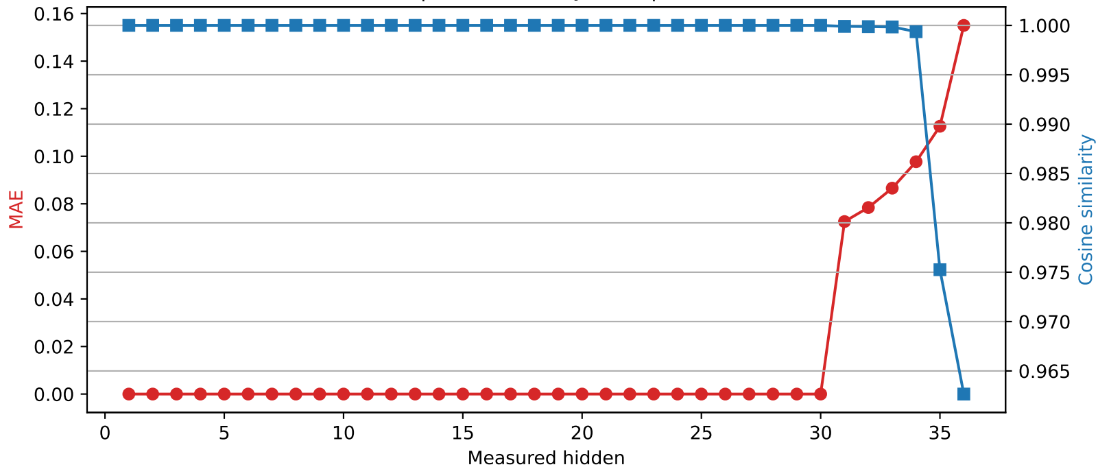
SmolLM3-3B | Quantized layer 30 | float16 → int2
