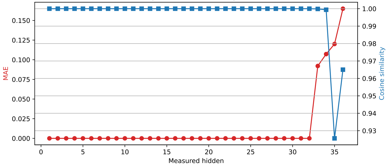
SmolLM3-3B | Quantized layer 32 | float16 → int2
